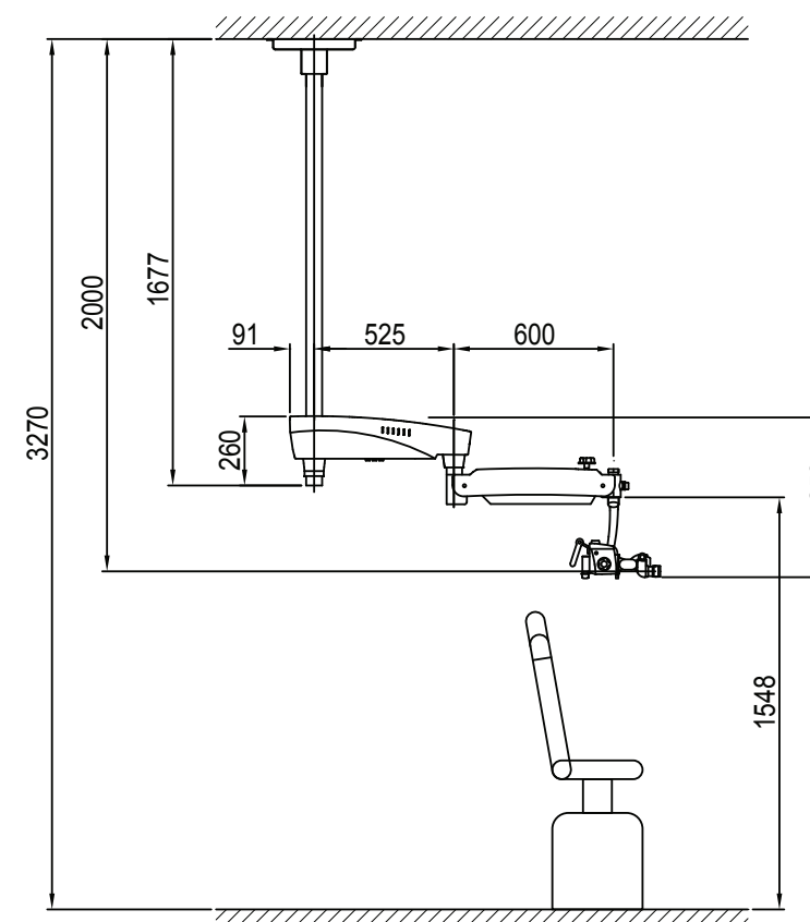
Ceiling Mount
